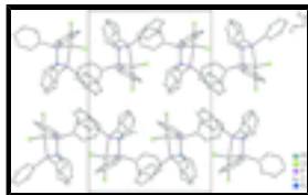
Fig. 2. Perspective view of the unit cell of the title compound along the a axis.
